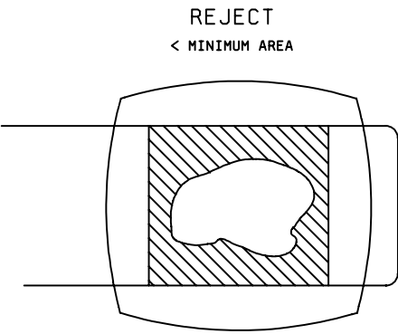
FIGURE 2035-3. Rejectable bond area.
