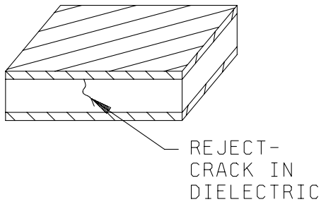
FIGURE 2032-61h. Class H crack in dielectric criterion.
