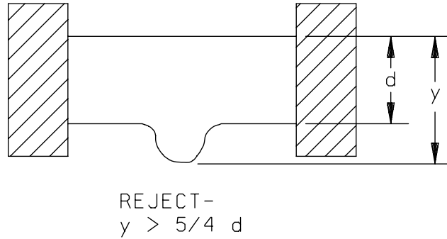
FIGURE 2032-20h. Class H resistor width increase criterion.
