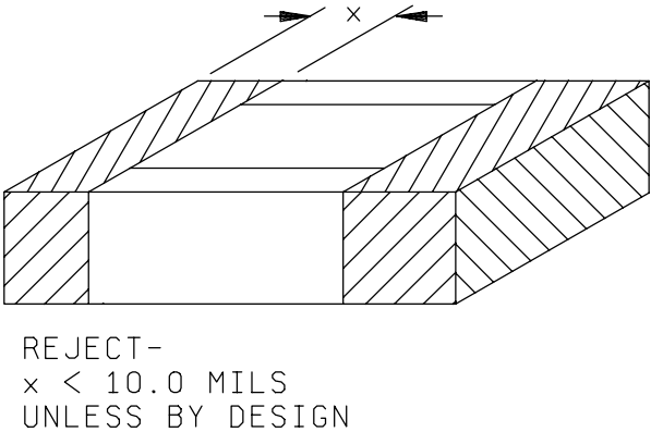
FIGURE 2032-63h. Class H termination width criterion.
