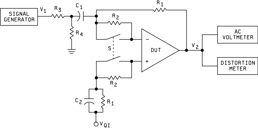
FIGURE 4004-1. Test figure for bandwidth and input impedance.
