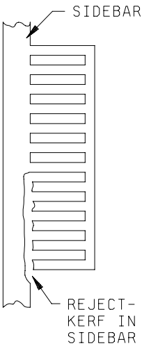
FIGURE 2032-30h. Class H resistor ladder sidebar trim criterion.
