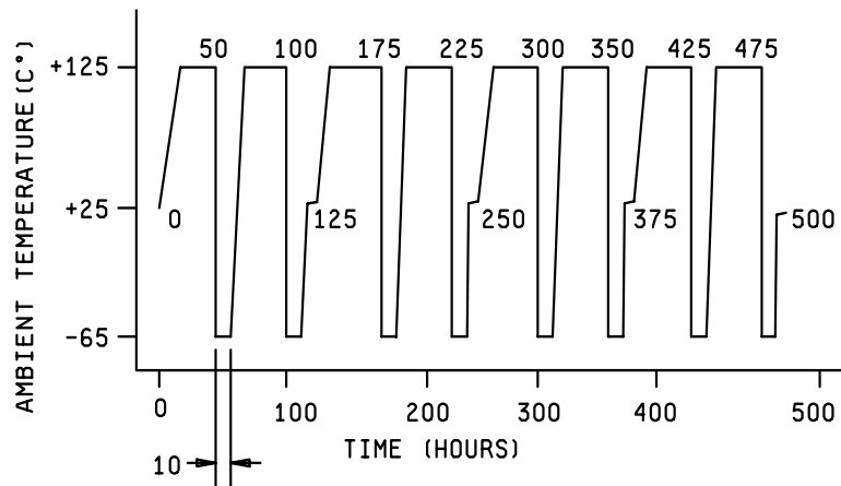
FIGURE 9. Coil life ambient temperatures.
