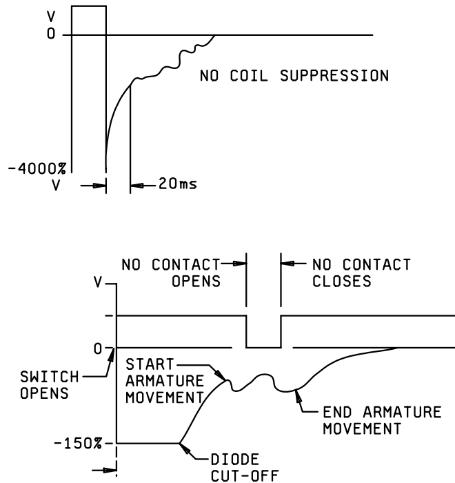
FIGURE 7. Typical transient voltage.
