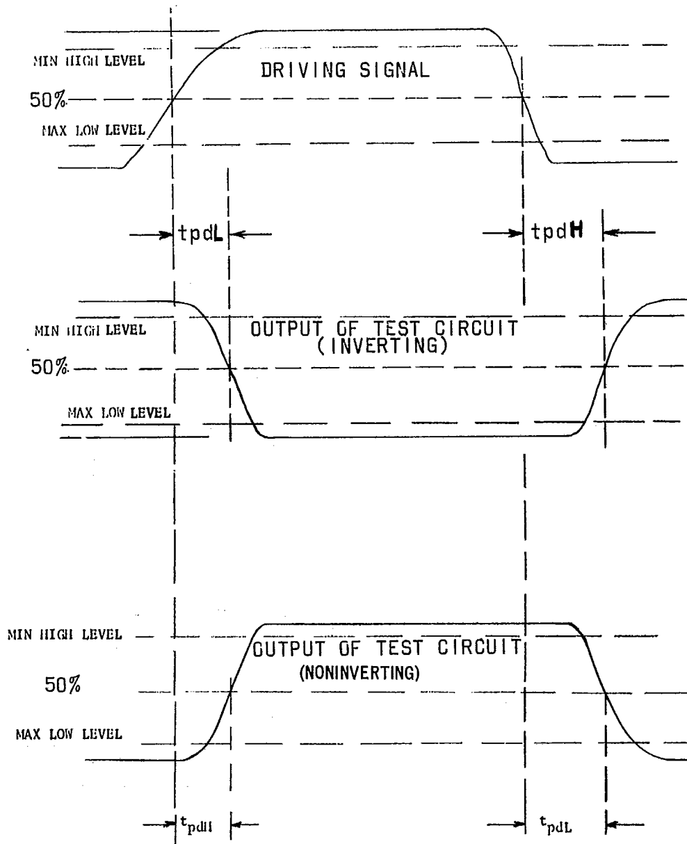
FIGURE 3003-2. Propagation delay.
