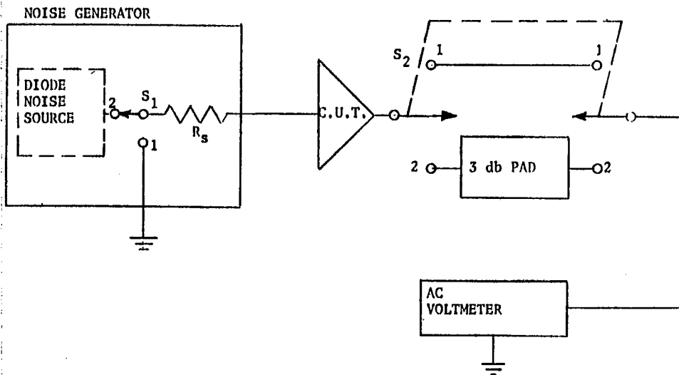
FIGURE 4006-4. Noise figure (double power technique).
