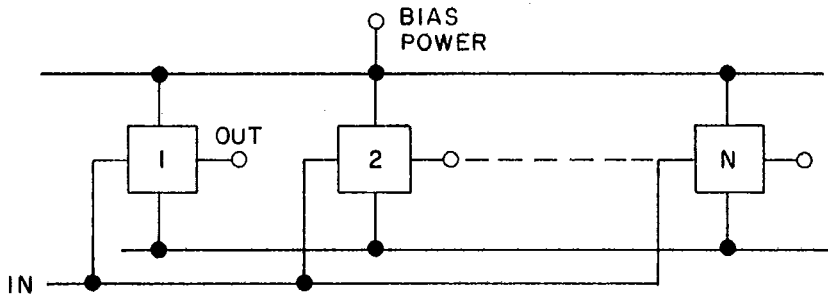
FIGURE 1005-2. Parallel excitation.
