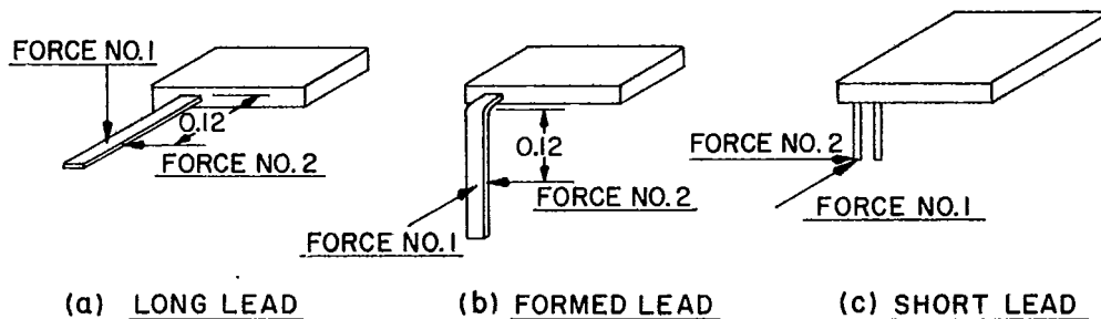
FIGURE 2004-1. Bending stress force application.
