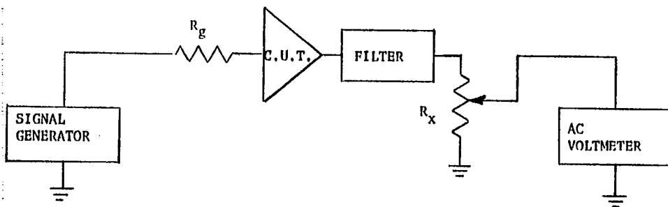
FIGURE 4006-3. Noise figure test circuit.
