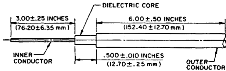
FIGURE 2. Stripping dimensions for semi-rigid cables.
