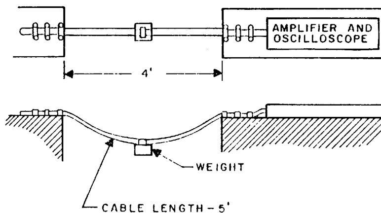
FIGURE 9. Equipment setup.
