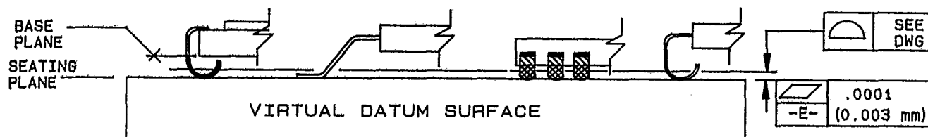
FIGURE 9. Coplanarity deviation .
