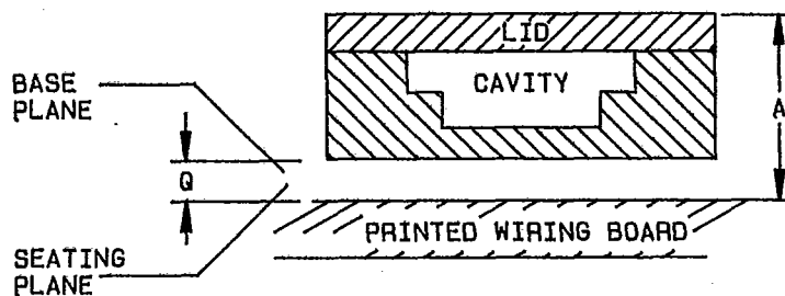
CAVITY-UP (TERMINALS NOT SHOWN)
