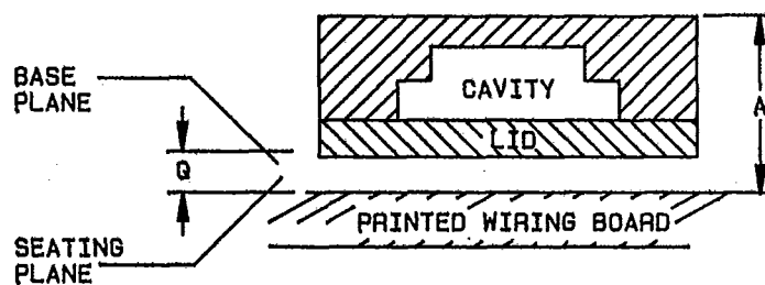
CAVITY-DOWN (TERMINALS NOT SHOWN)
