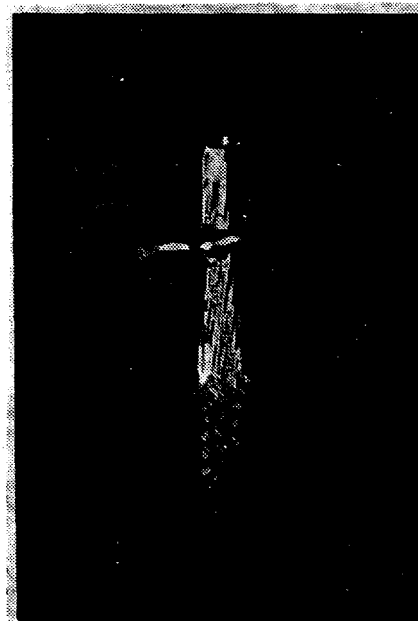
FIGURE 208-4. Illustration of acceptable solderable stranded wire.
