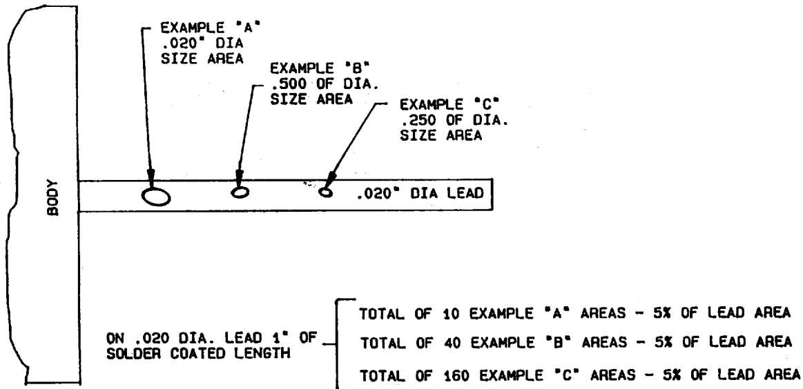
FIGURE 208-6. Aid in evaluation of 5 percent allowable defect area - Continued.
