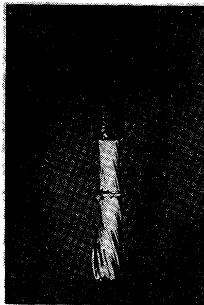
FIGURE 208-5. Illustration of partially solderable stranded wire showing incomplete fillet.
