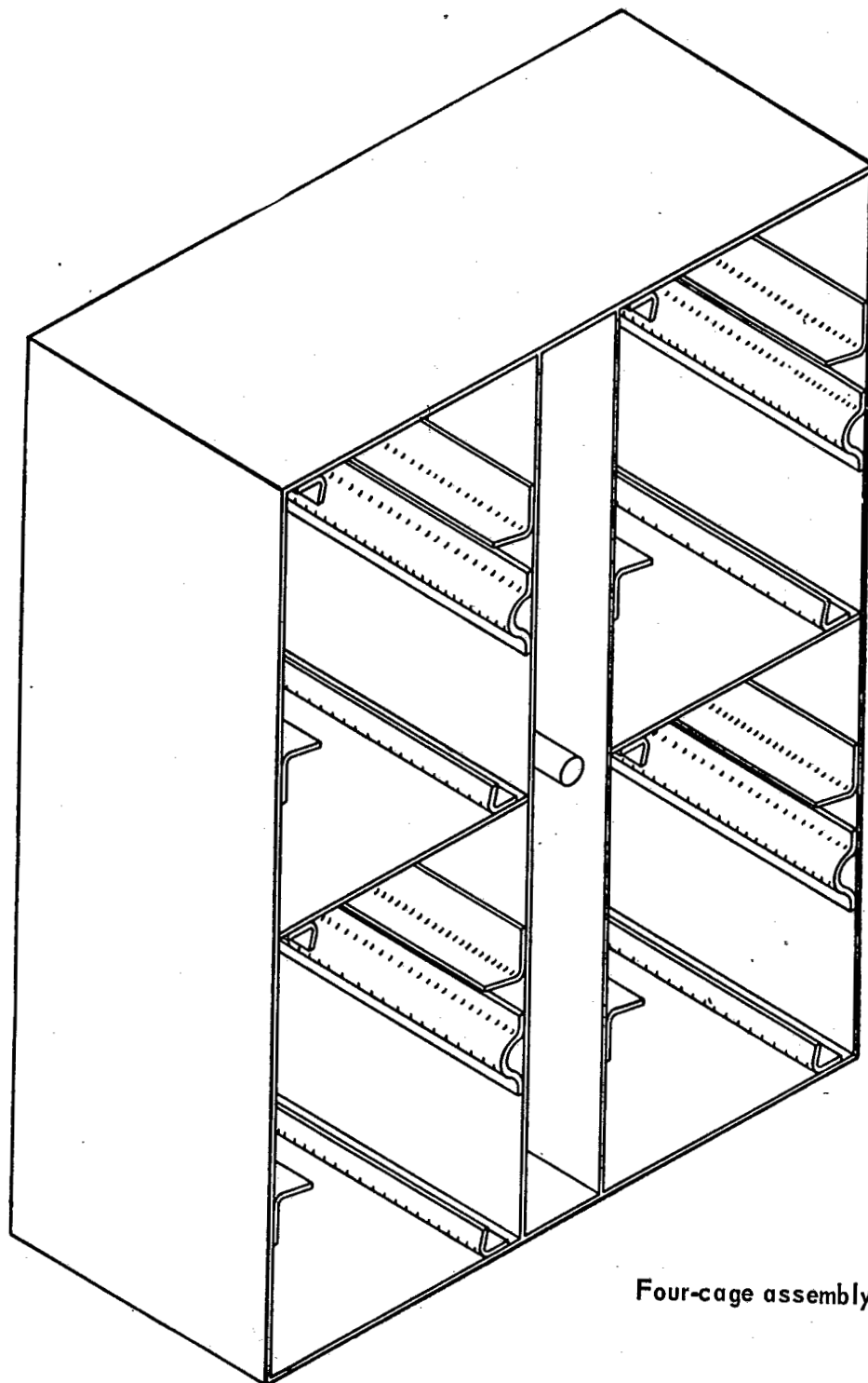
FIGURE 203-2. Cage assembly.
