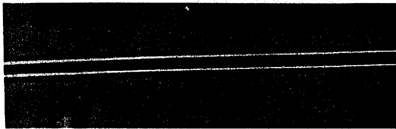
FIGURE 208-8A. Photograph 2 - acceptable soldering coating - very small percentage of area covered by pinholes or defects.
