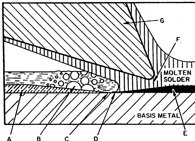
FIGURE 1. Solder iron process diagram.
