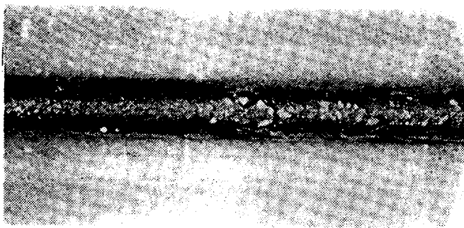
FIGURE 208-1. Nonwetting.
