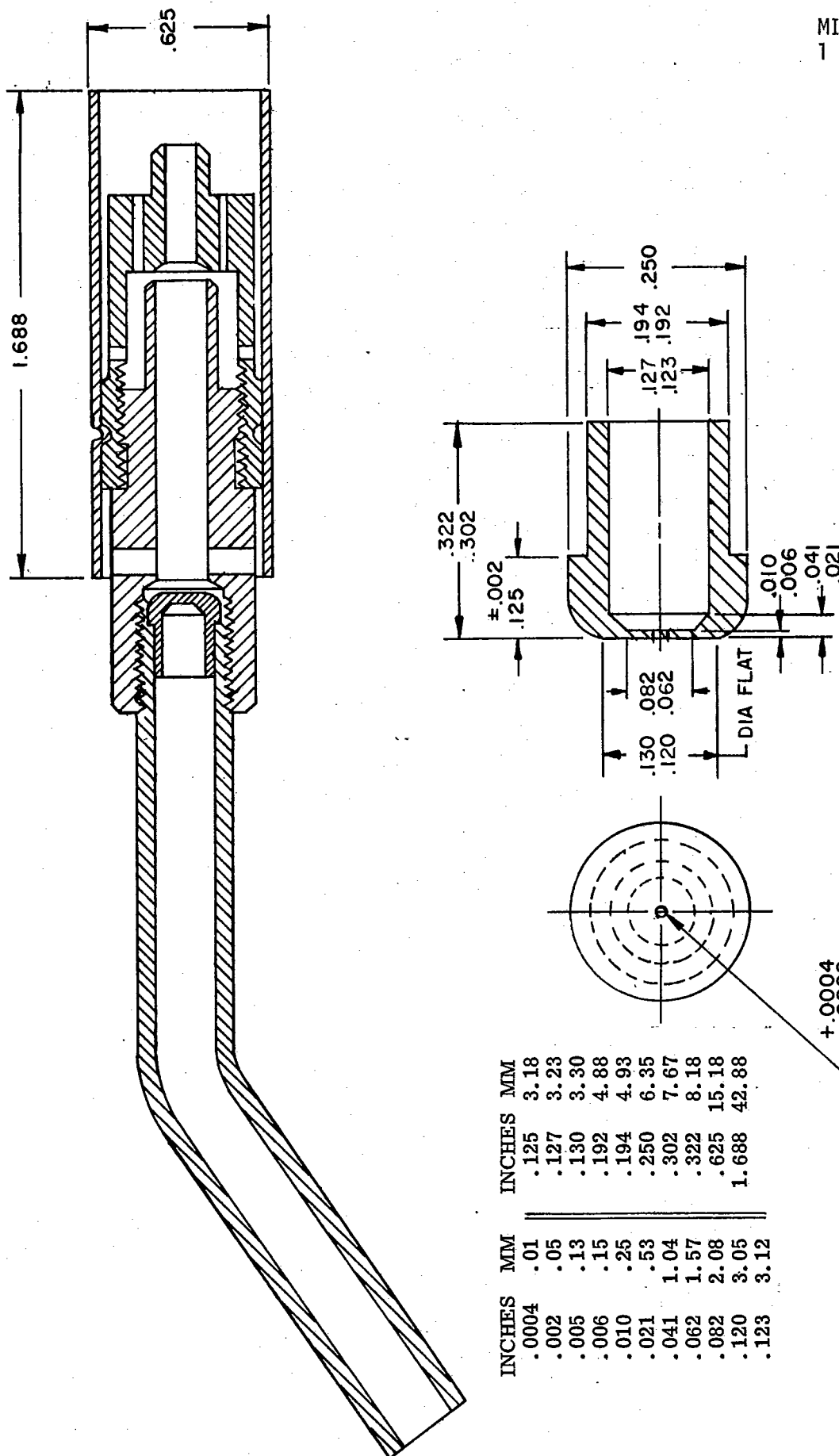
FIGURE 111-1. Burner head.
