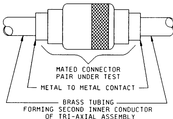
FIGURE 6A. Connector assembly for RF leakage test.
