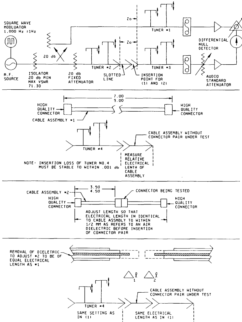
FIGURE 7. Method of insertion loss measurement of rated connector pair.
