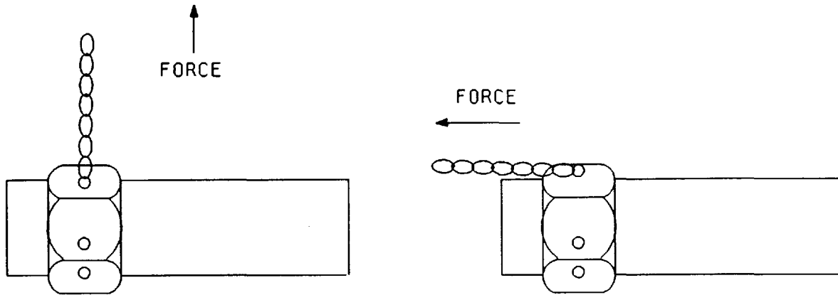
FIGURE 8. Safety wire hole pullout procedure.
