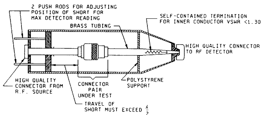
FIGURE 6B. RF leakage test set-up.
