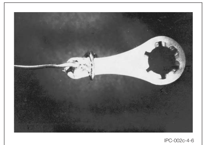
Figure 4–6 Illustration of Unsolderable Terminal
