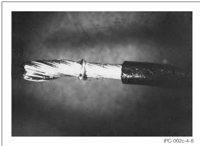
Figure 4-8 Illustration of Partially Solderable Stranded Wire Showing Incomplete Fillet
