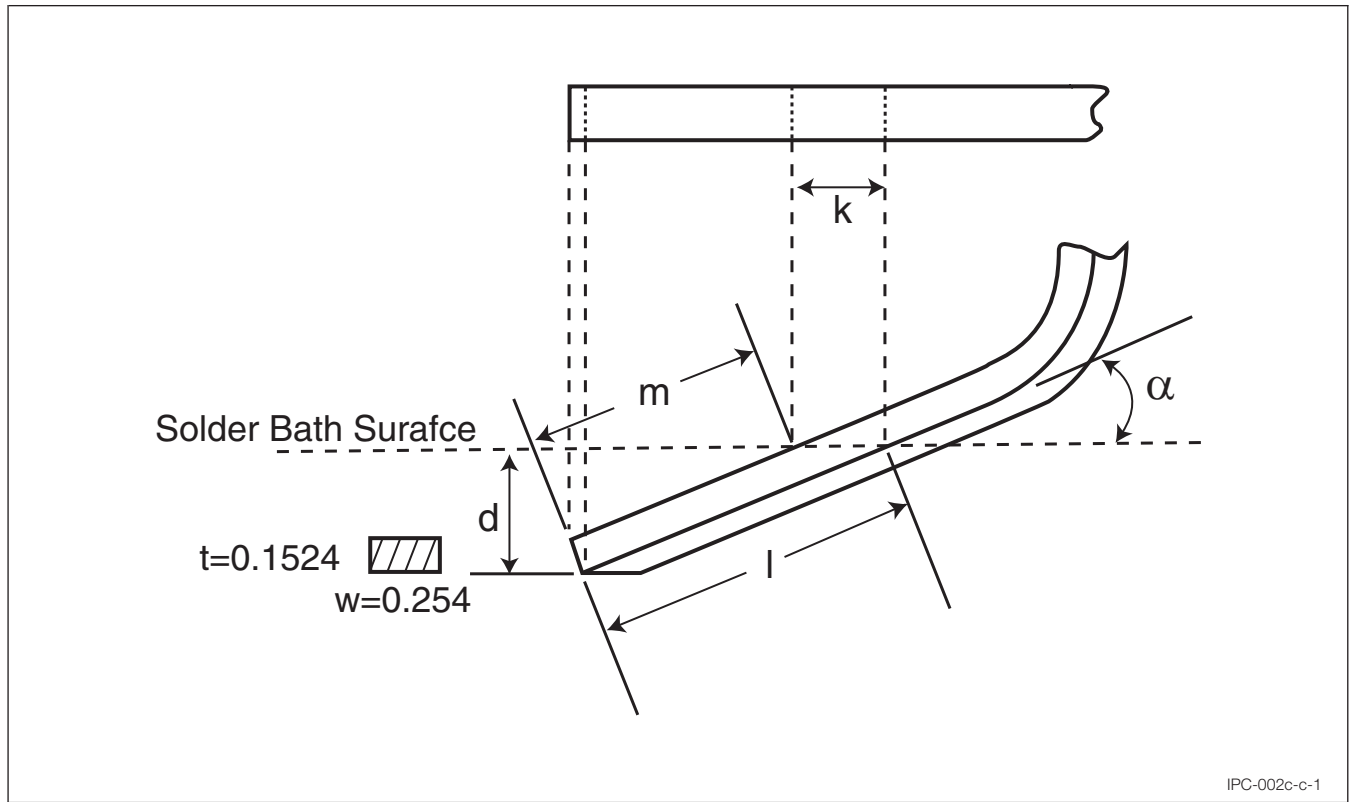
Figure C-1 Lead Periphery and Volume for a 132 I/O PQFP
