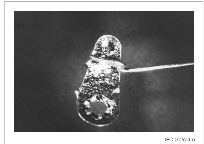
Figure 4–5 Illustration of Acceptable Solderable Terminal
