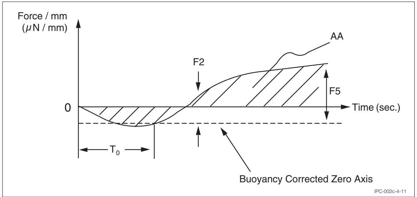
Figure 4-11 Set B Wetting Curve
