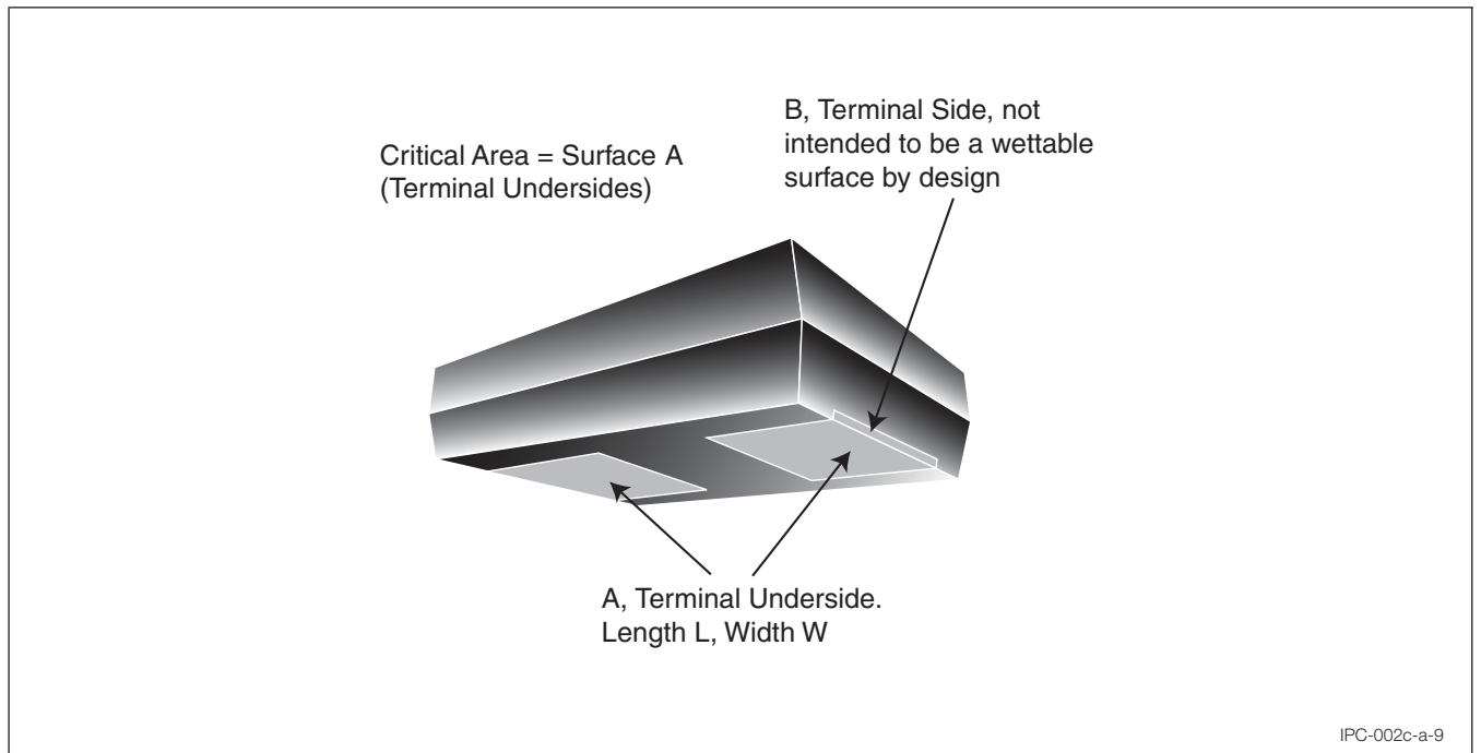
Figure A-9 Bottom-Only Termination Component
