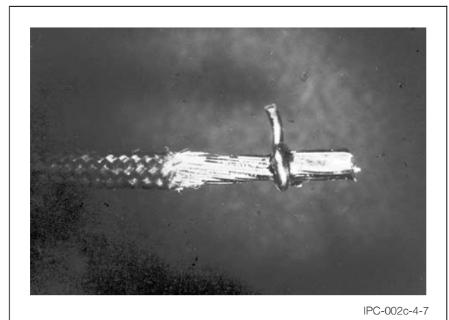
Figure 4–7 Illustration of Acceptable Solderable Stranded Wire
