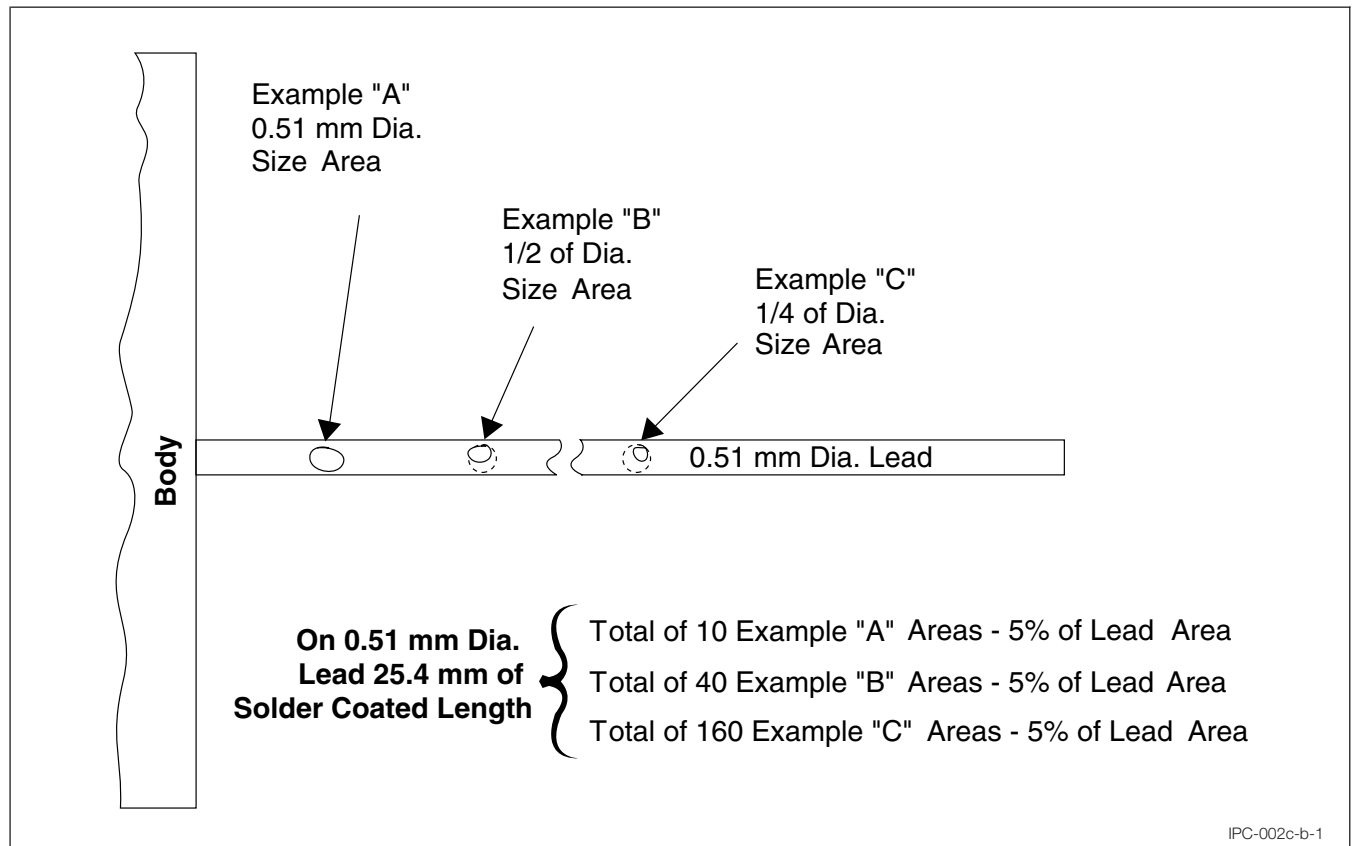
Figure B-1 Defect Size Aid
