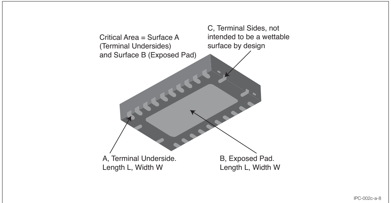
Figure A-8 Exposed Pad Package
