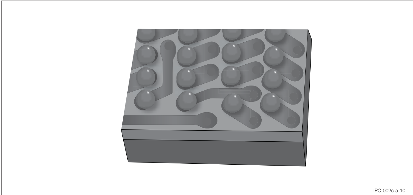
Figure A-10 Area Array Component Critical Surface
