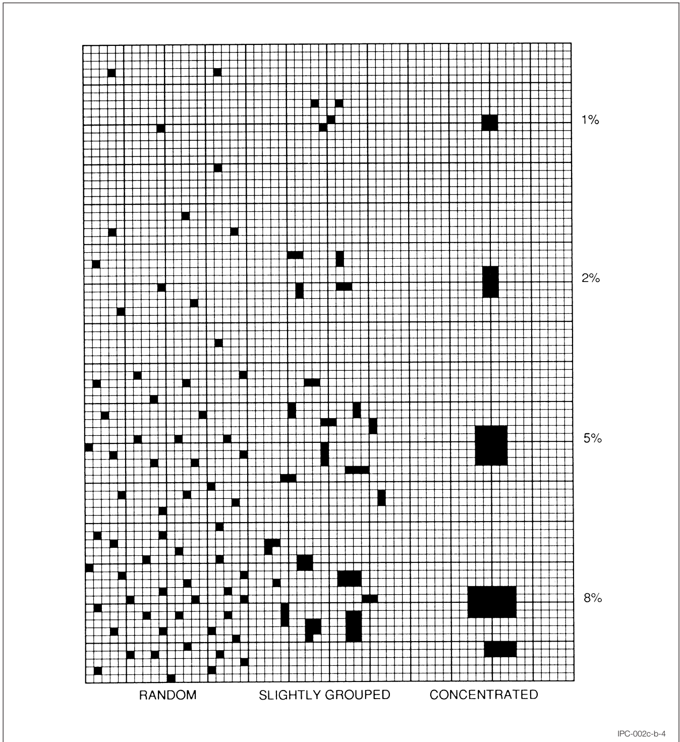
Figure B-4 Aid in Evaluation of 5% Allowable Area of Pin Holes
