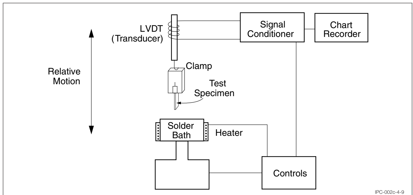
Figure 4–9 Wetting Balance Apparatus
