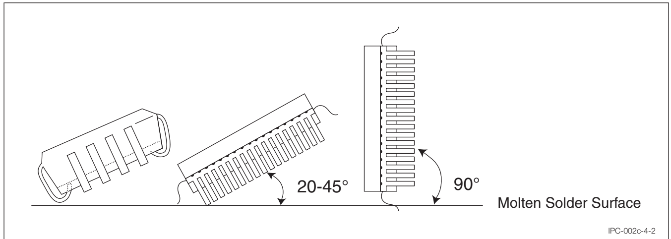
Figure 4-2 Solder Dipping Angle for Surface Mount Ledged Components
