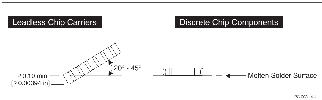
Figure 4–4 Leadless Component Immersion Depth
