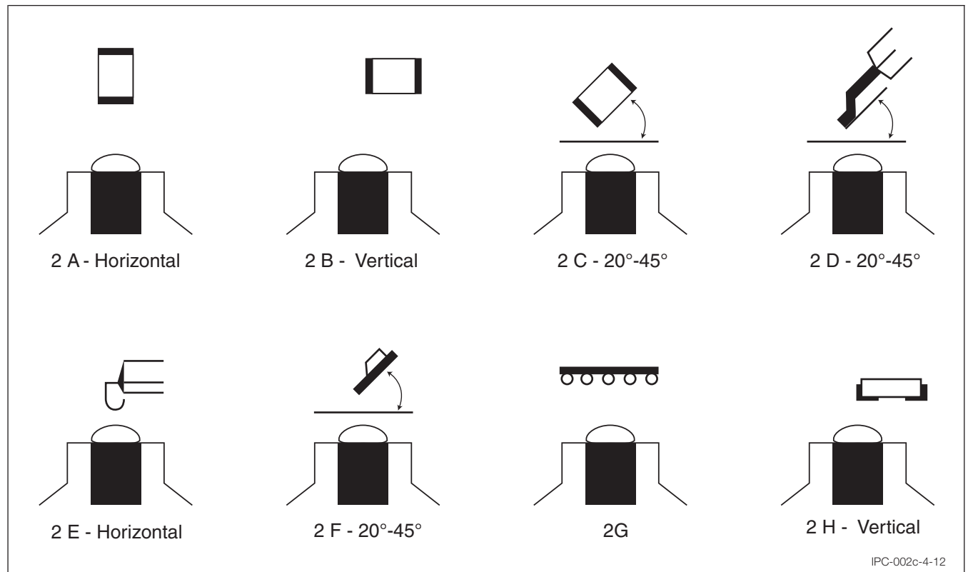
Figure 4-12 Component and Dipping Angle (Directly from IEC 60068-2-69)
