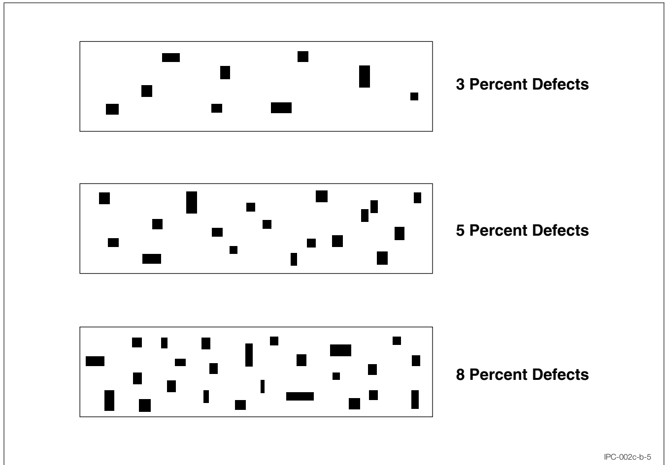
Figure B-5 Solderability Coverage Guide
