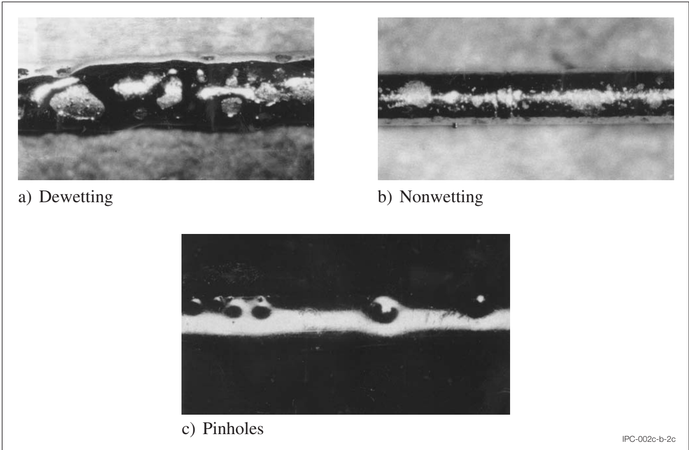
Figure B-2 Types of Solderability Defects
