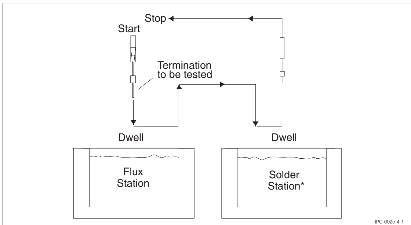
Figure 4-1 Dipping Schematic
