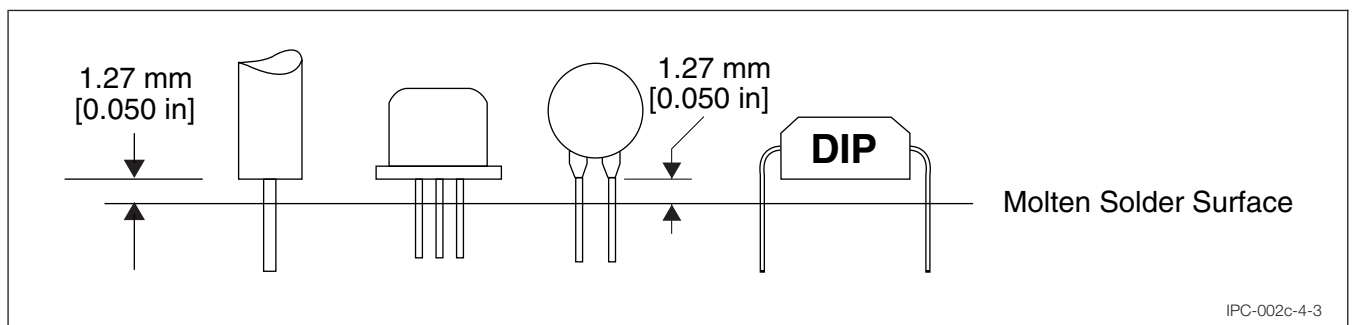
Figure 4-3 Solder Dipping Depth for Through-Hole Components
